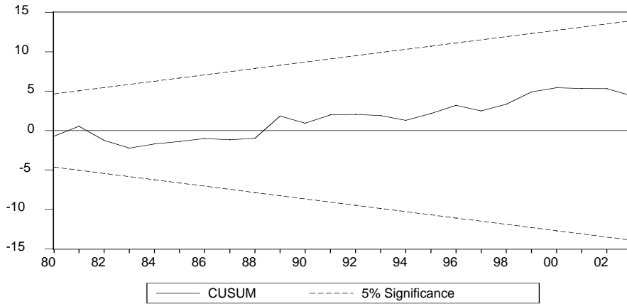
FIGURE 1 CUSUM
