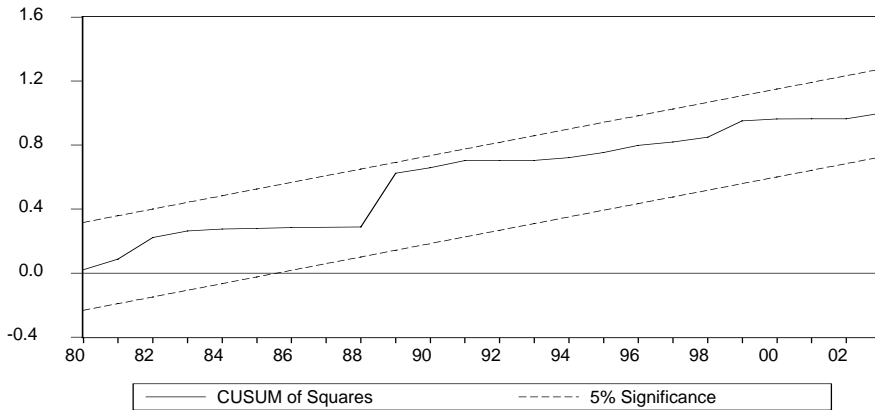
FIGURE 2 CUSUM SQ
